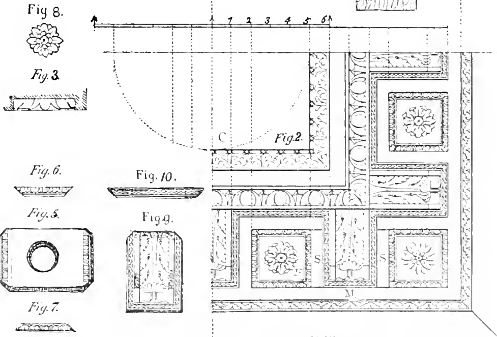
ELEVATION OF CORINTHIAN ENTABLATURE AND PLAN OF CORNICE AT EXTERNAL ANGLE.
